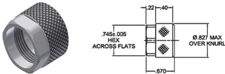
Figure 2. Knurled/Hex Coupling Nut Change
