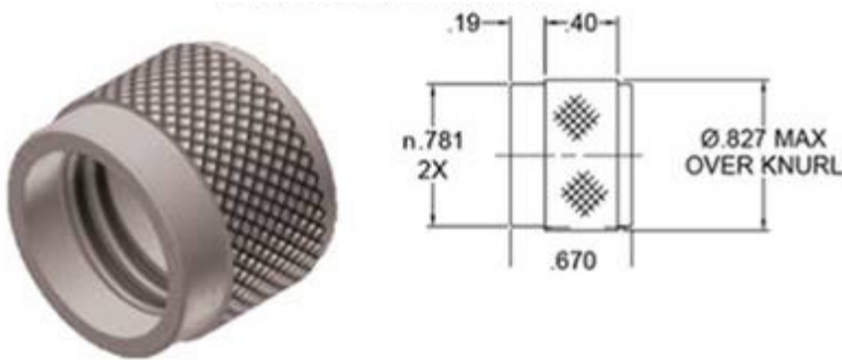
Figure 1. Knurled Coupling Nut
