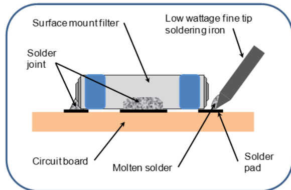
Figure 2 – Solder Recommendations Surface Mount Filters
