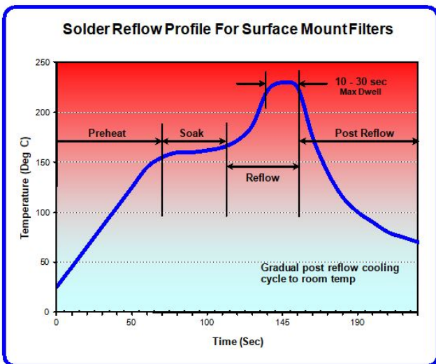
Figure 1 – Typical Solder Reflow Profile for Surface Mount Filter Assemblies
