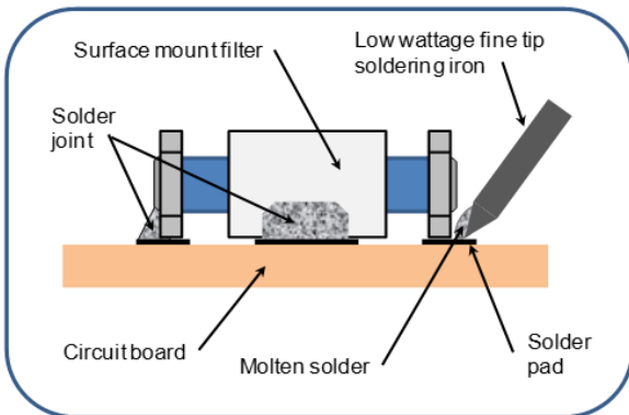
Figure 2 – Solder Recommendations Surface Mount Filters
