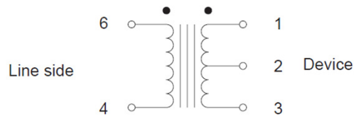
TEW4921 & -1
