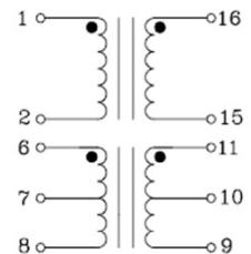
SCHEMATIC 2
