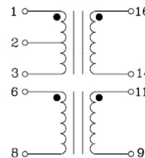
SCHEMATIC 1
