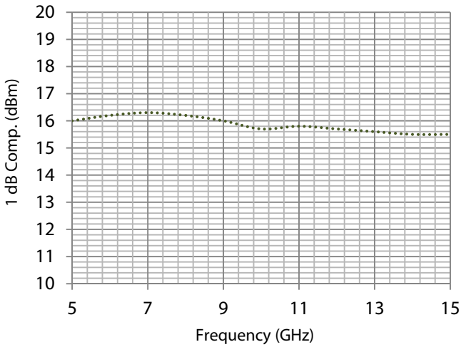
1 dB Compression (dBm)
