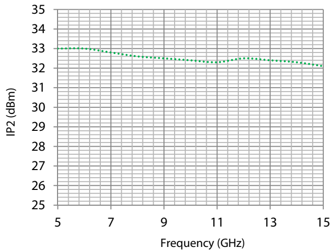
2 nd Order Intercept (dBm)
