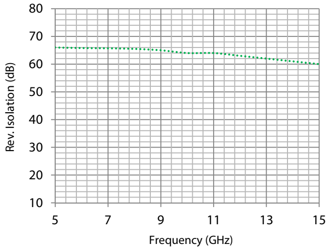
Reverse Isolation (dB)
