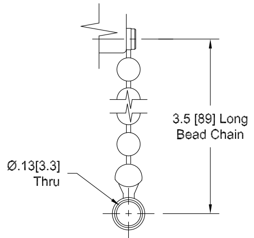
CHAIN DETAIL
