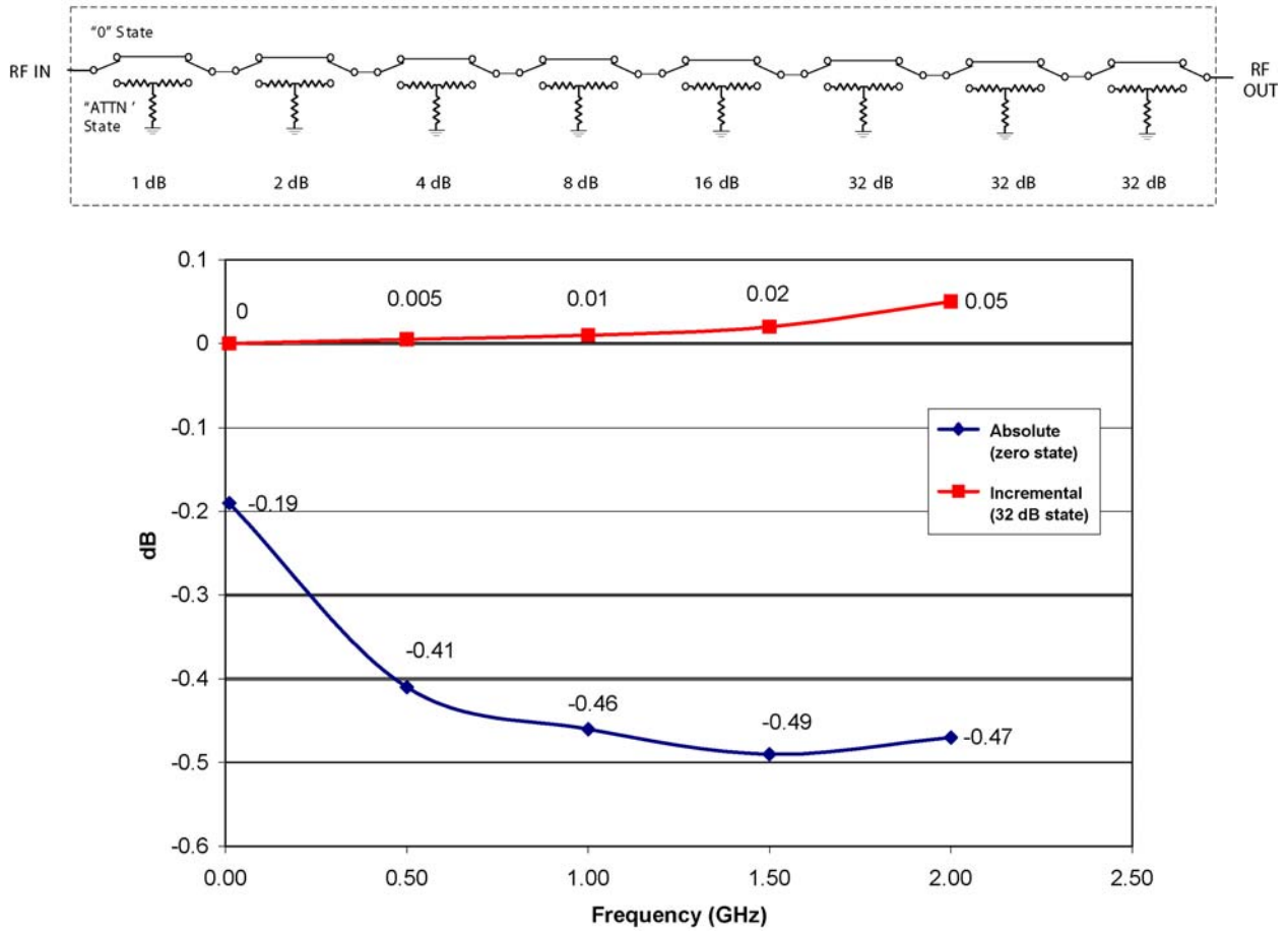
Figure 4 -- 8 Cell Relay-Based Programmable Attenuator Change in the Absolute and Incremental Attenuation from 25 °C to 100 °C
