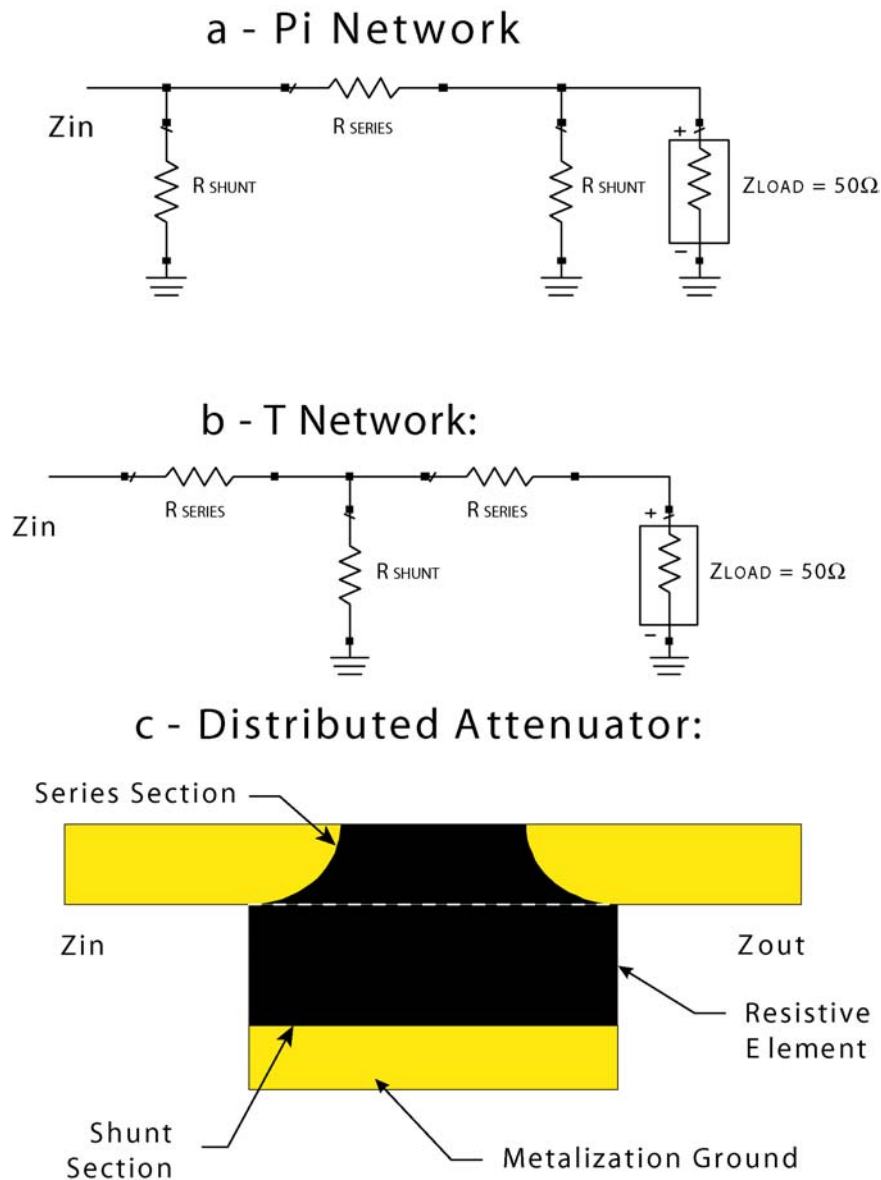
Figure 1. PI and T Network Schematics
